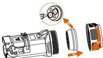
3 Loosen the swivel nut, pull out the rubber stopper out of the AC connector. Scratch the ports of the rubber stopper with a knife.
