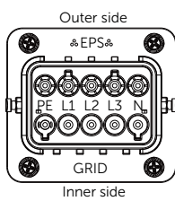
9 Remove the dustproof cover from the Grid&EPS port.
