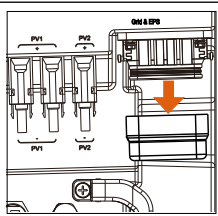
9 Remove the dustproof cover from the Grid&EPS port.
