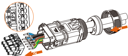
5 Plug L1/ L2/ L3/ N/ PE cables into the corresponding ports of the terminal block.
