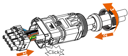
7 Insert the terminal block and rubber stopper back to the AC connector and tighten the swivel nut.
